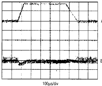
LINE-TRANSIENT RESPONSE (12V AUXILIARY SMPS)
