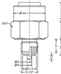
Type 9 – Thread ISO 228-1 – G½”B, front-flush
