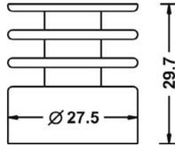
Type 4 – Thread ISO 228-1 – G¼”I, inner thread
