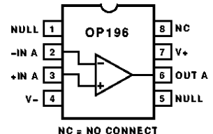
8-Lead Epoxy DIP (P Suffix)
