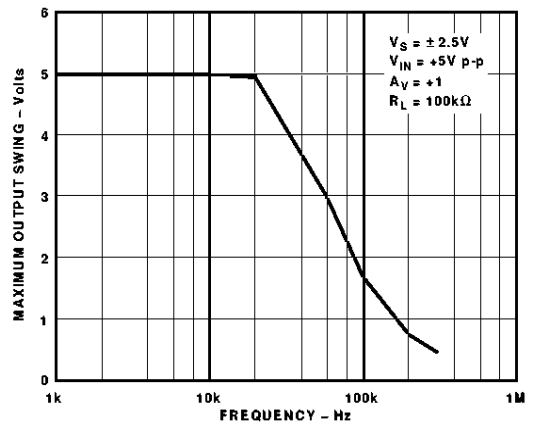
Figure 24. Maximum Output Swing vs. Frequency
