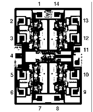
OP496 Die Size 0.062 × 0.092 inch, 5,704 sq. mils Substrate (Die Backside) Is Connected to V+. Transistor Count, 214.
