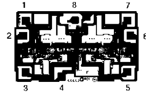
OP296 Die Size 0.072 × 0.0048 inch, 3,456 sq. mils Substrate (Die Backside) Is Connected to V+. Transistor Count, 110.
