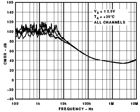
Figure 22. CMRR vs. Frequency
