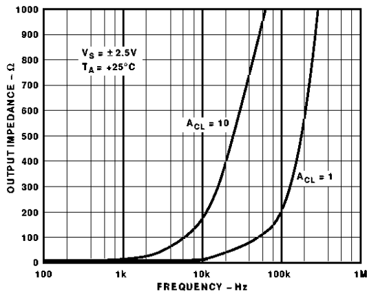
Figure 21. Output Impedance vs. Frequency
