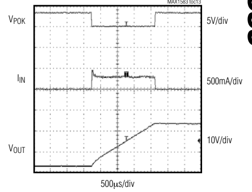
PRECHARGE-CYCLE WAVEFORMS (MAX1583Y)
