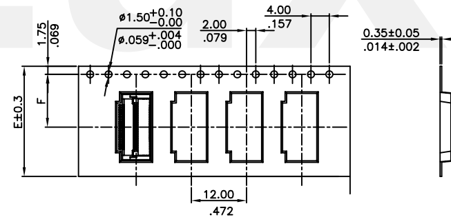
WIDTH : 24 mm Carrier (SCALE 1:4)
