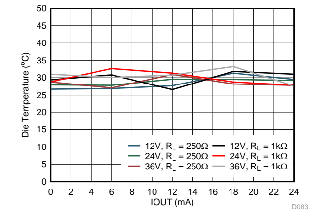
Figure 85. IOU Die Temperature vs Load
