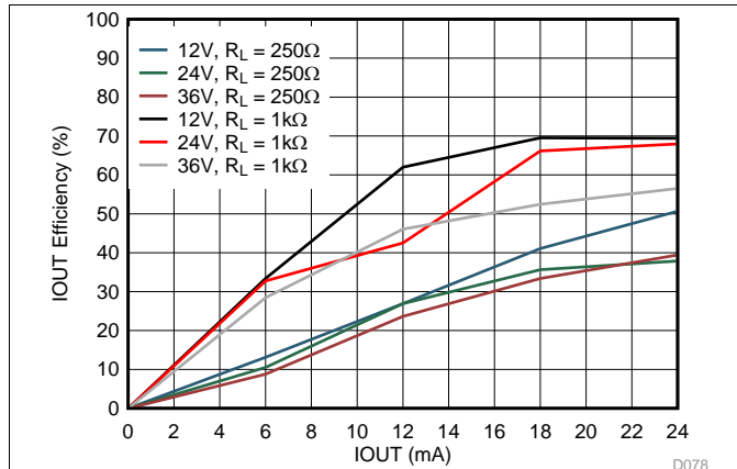
Figure 80. IOU DC/DC Efficiency
