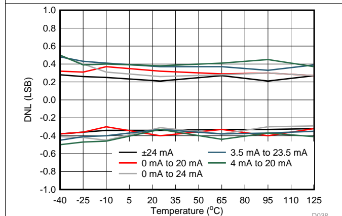
Figure 42. IOUT DNL vs Temperature
