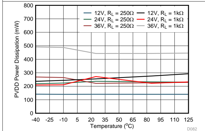
Figure 84. IOU Power Dissipation vs Temperature
