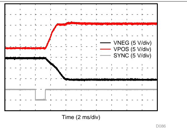
Figure 87. VOUT Enable VPOS and VNEG Settling Time
