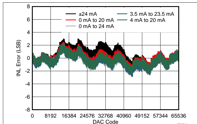
Figure 38. IOUT INL vs Code (DC/DC Disabled)
