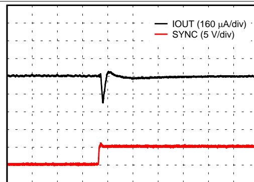
Figure 57. IOUT Settling Time, Bipolar Range, Rising Signal
