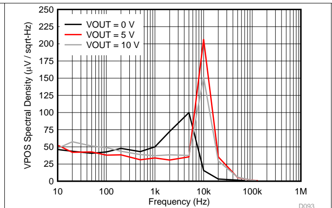
Figure 93. VOUT VPOS Noise Spectral Density
