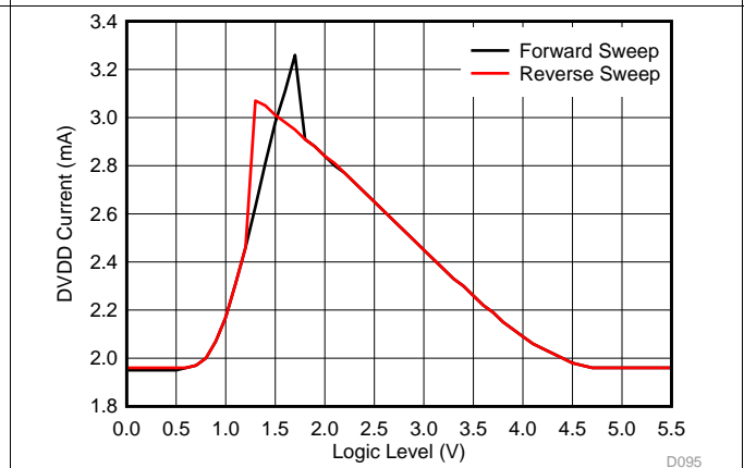
Figure 95. DVDD Iq vs Logic Level
