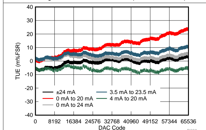
Figure 40. IOUT TUE vs Code (DC/DC Enabled)
