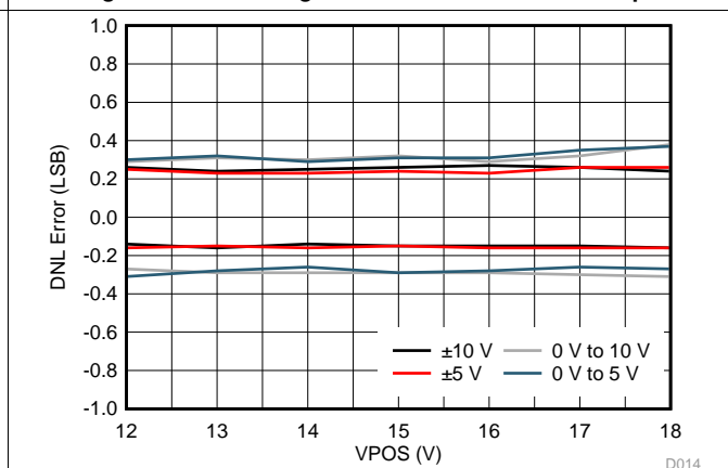
Figure 18. VOUT DNL vs VPOS
