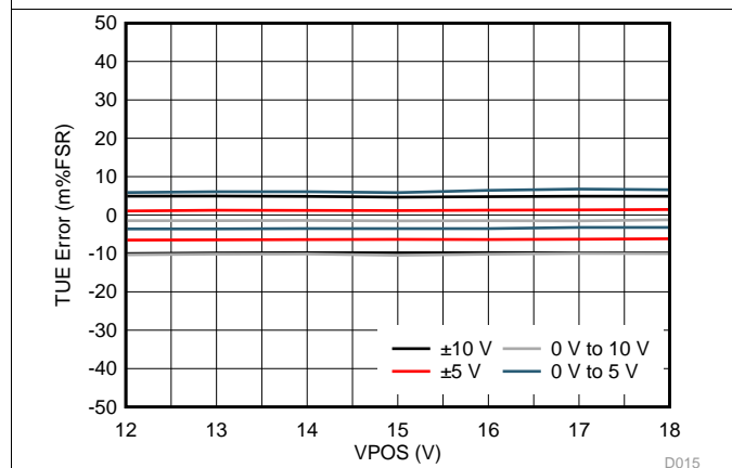
Figure 19. VOUT TUE vs VPOS
