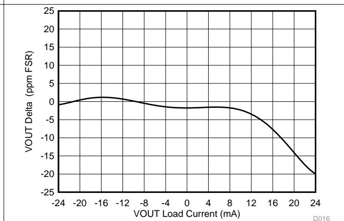
Figure 20. VOUT Load Regulation (SCLM = 11)
