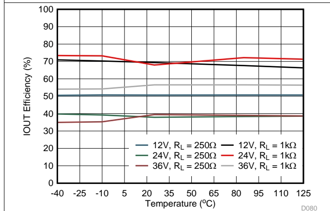
Figure 82. IOU DC/DC Efficiency vs Temperature
