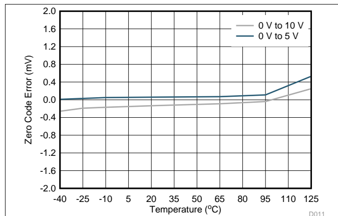
Figure 15. VOUT Zero-Code Error vs Temperature
