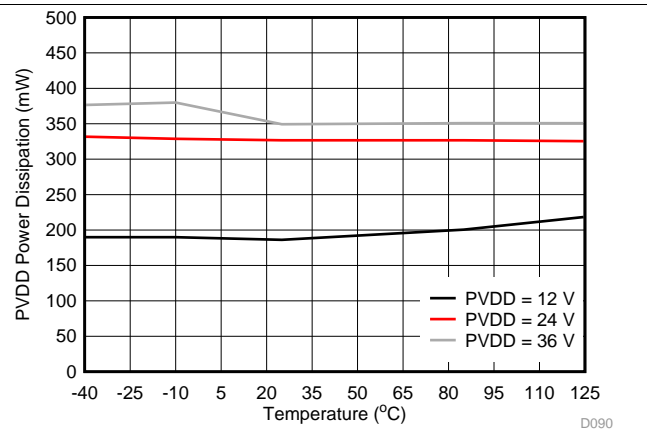
Figure 91. VOUT Power Dissipation vs Temperature
