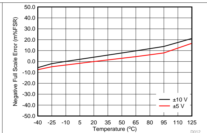
Figure 16. VOUT Negative Full-Scale Error vs Temperature
