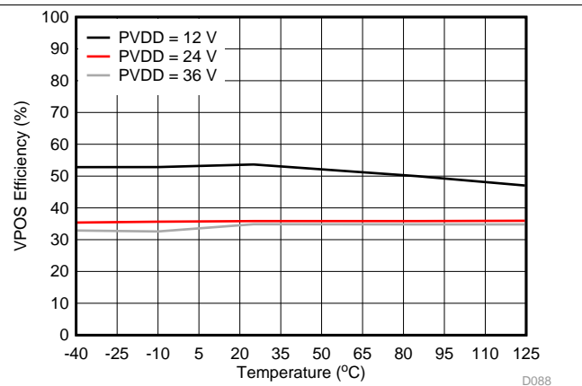
Figure 89. VOUT VPOS Efficiency vs Temperature
