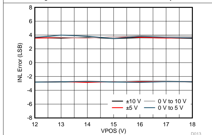
Figure 17. VOUT INL vs VPOS
