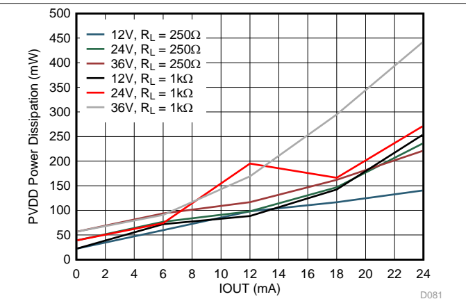
Figure 83. IOU Power Dissipation vs Load
