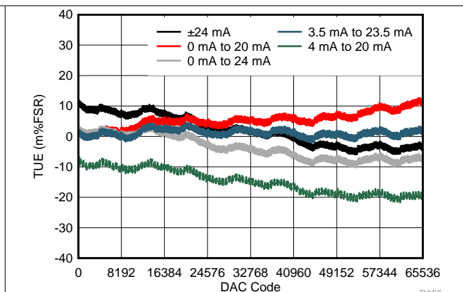
Figure 39. IOUT TUE vs Code (DC/DC Enabled)
