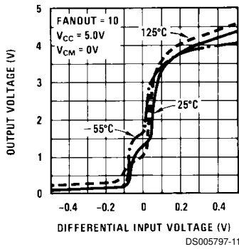
Transfer Function
