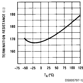
Termination Resistance
