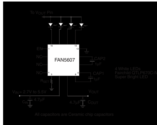
Figure 1. Test Circuit
