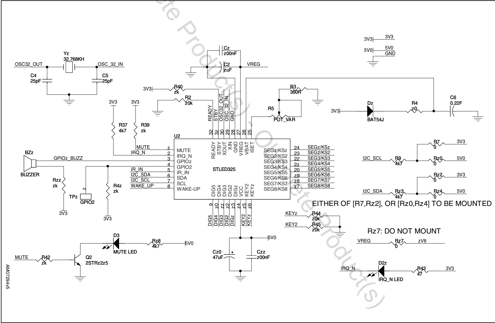
Figure 3. STEVAL-ILL029V: STLED325
