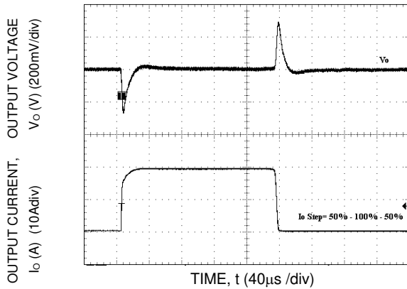
Figure 16. Transient Response to Dynamic Load Change from 0% to 50% to 100% to 50% to 0% with V_{IN}=12V .
