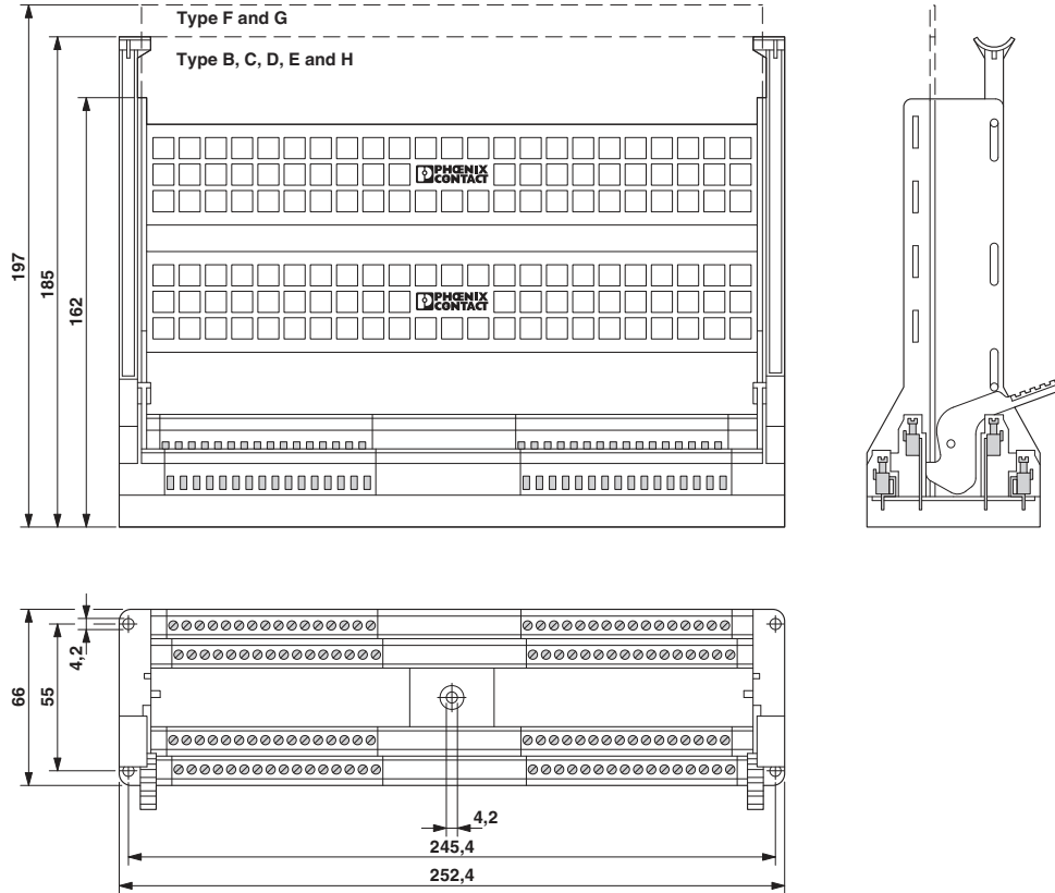
Dimensioned drawing
