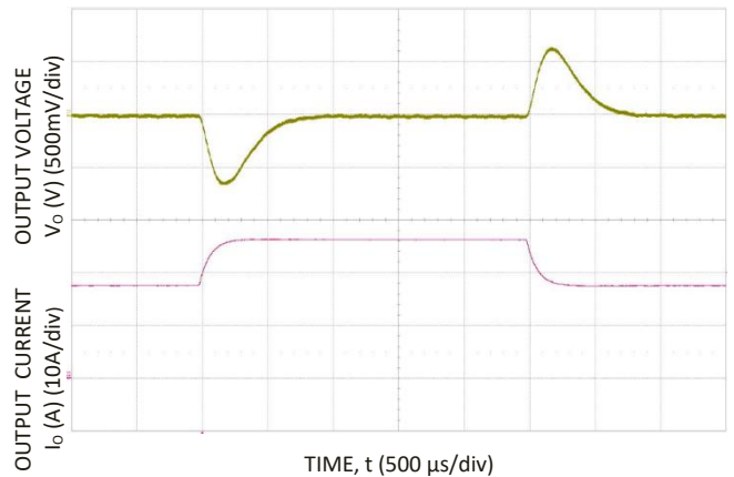
Figure 4. Typical Transient Response to 0.1A/ \mu s Step Change in Load from 50% to 75% to 50% of Full Load, C_o = 470\mu F and 48 Vdc Input.
