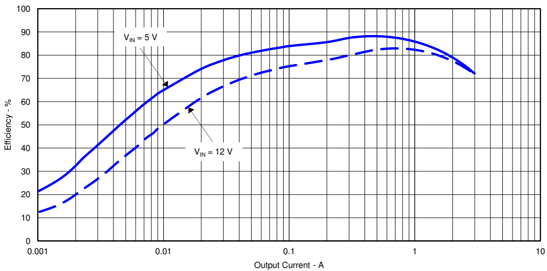
Figure 4-2. TPS54339EEVM-056 Light-Load Efficiency
