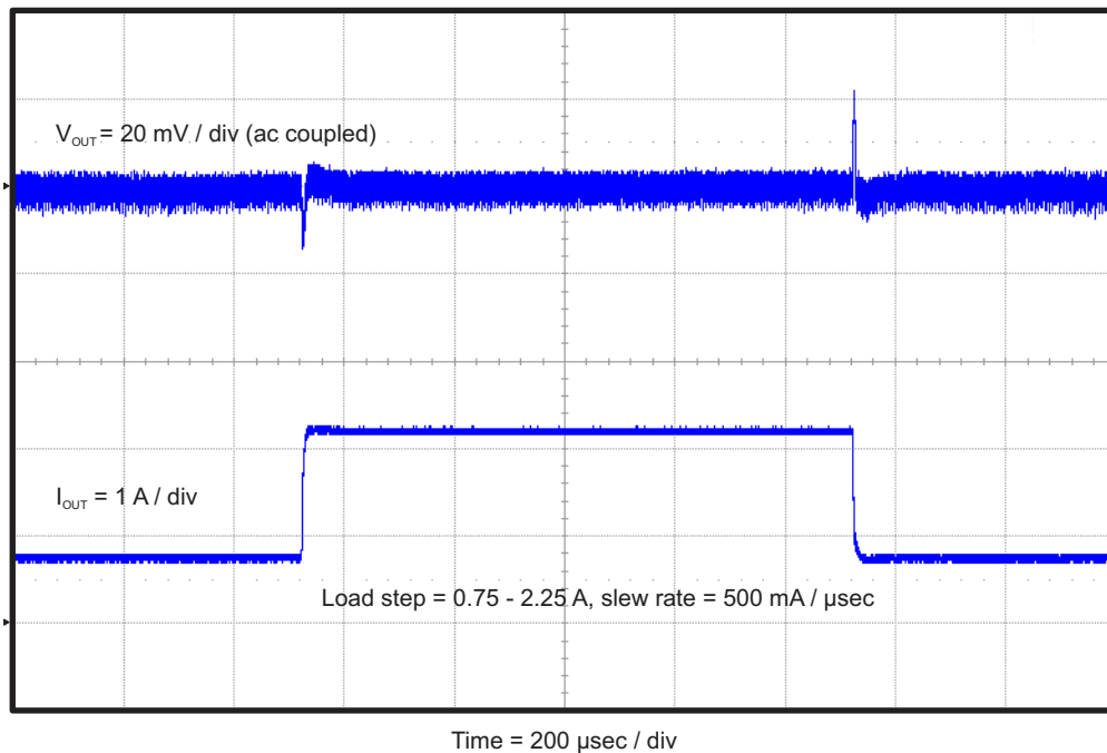
Figure 4-6. TPS54339EEVM-056 Load Transient Response
