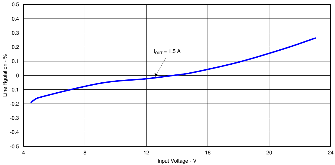
Figure 4-4. TPS54339EEVM-056 Line Regulation
