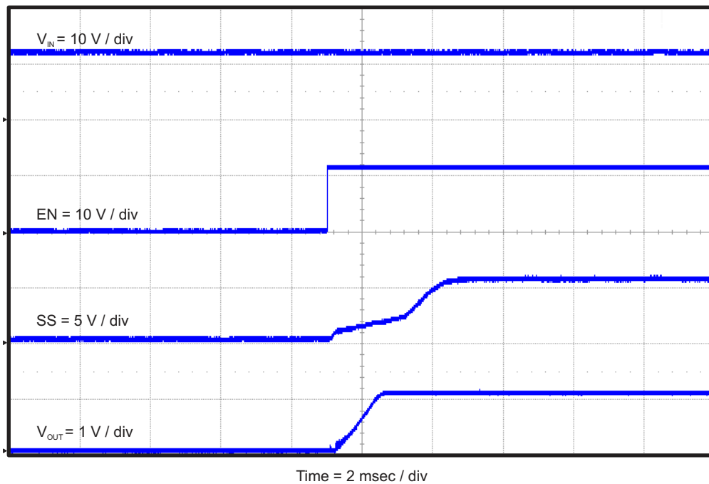
Figure 4-12. TPS54339EEVM-056 Start-Up Relative to EN with SS
