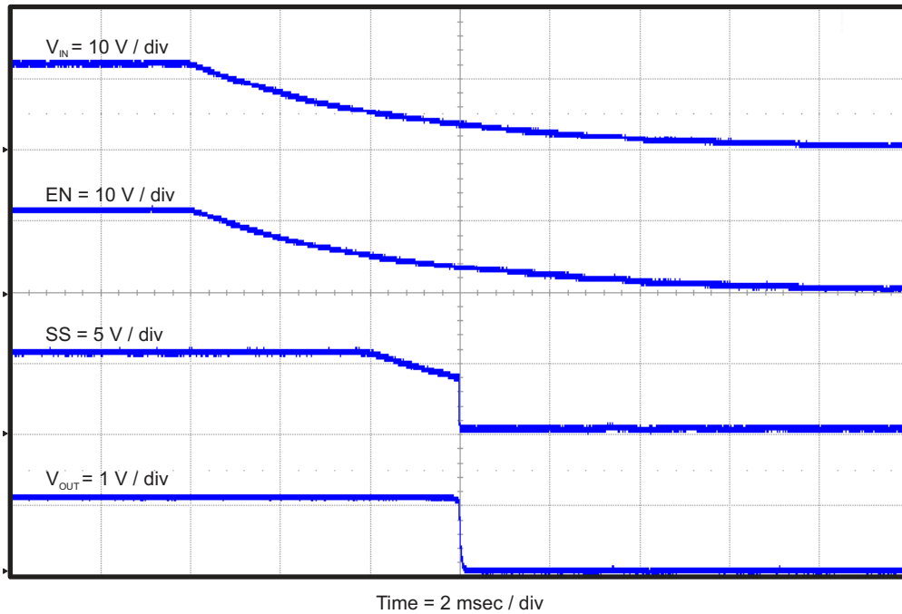
Figure 4-13. TPS54339EEVM-056 Shut-Down Relative to V_{IN} with SS
