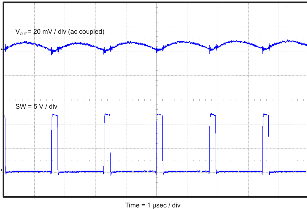
Figure 4-7. TPS54339EEVM-056 Output Voltage Ripple ( I_{OUT} = 3 A)
