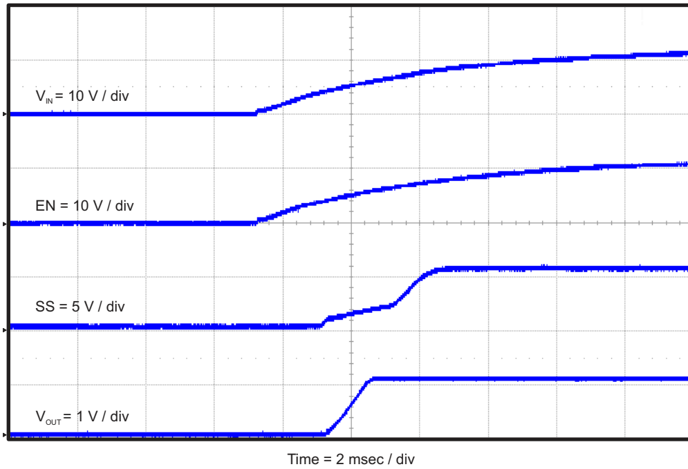
Figure 4-11. TPS54339EEVM-056 Start-Up Relative to V_{IN} with SS
