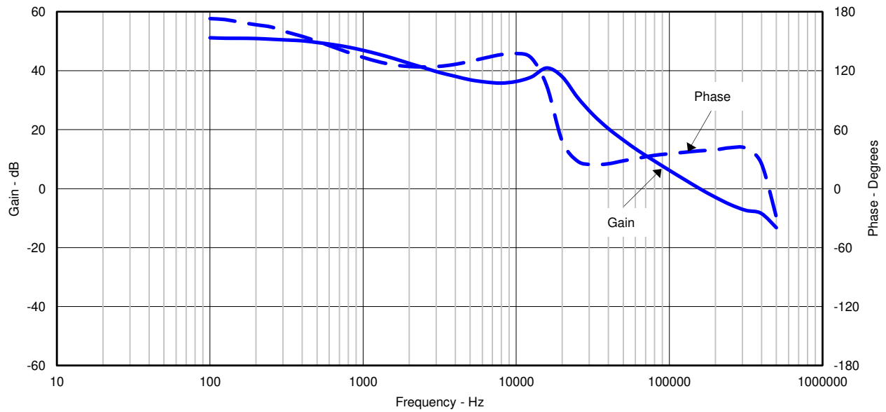
Figure 4-5. TPS54339EEVM-056 Closed Loop Response
