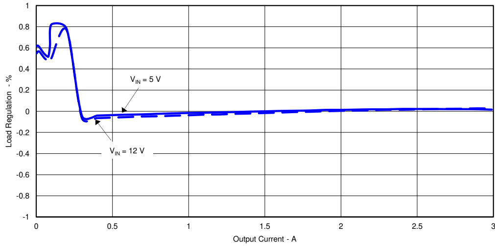
Figure 4-3. TPS54339EEVM-056 Load Regulation, V_{IN} = 5\text{ V} and V_{IN} = 12\text{ V} .
