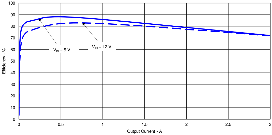
Figure 4-1. TPS54339EEVM-056 Efficiency
