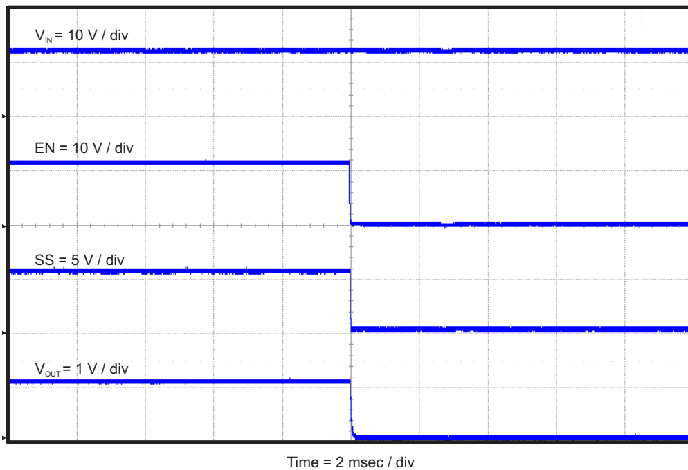
Figure 4-14. TPS54339EEVM-056 Shut-Down Relative to EN with SS
