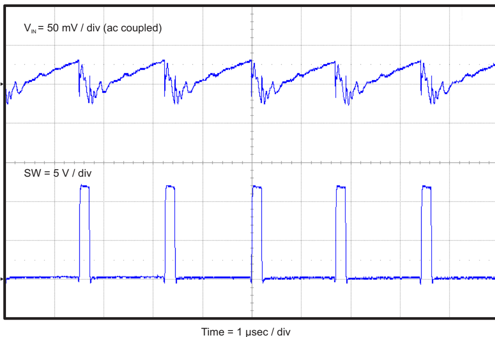
Figure 4-10. TPS54339EEVM-056 Input Voltage Ripple
