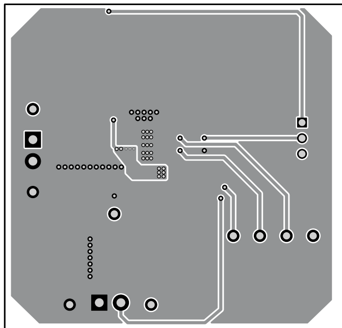
Figure 5-5. Bottom Layer
