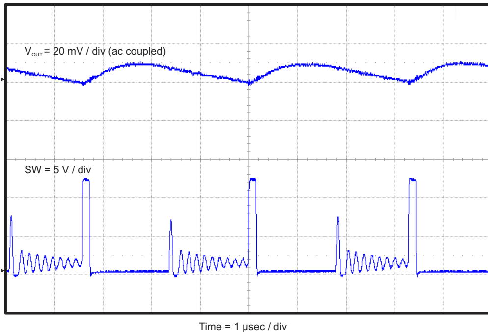
Figure 4-8. TPS54339EEVM-056 Output Voltage Ripple ( I_{OUT} = 150 mA)
