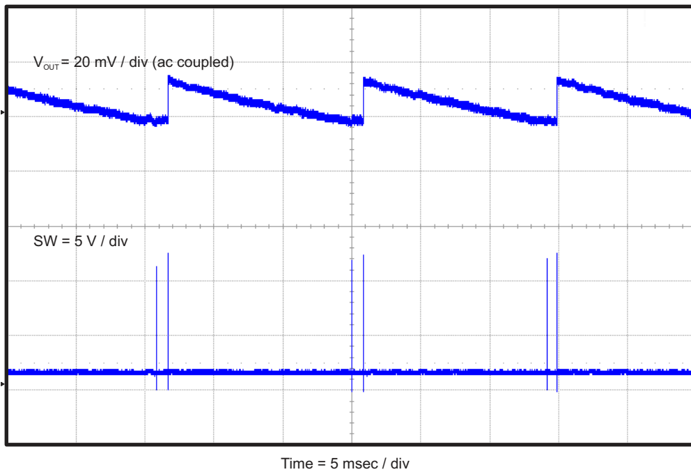
Figure 4-9. TPS54339EEVM-056 Output Voltage Ripple ( I_{OUT} = 0 \text{ A} )
