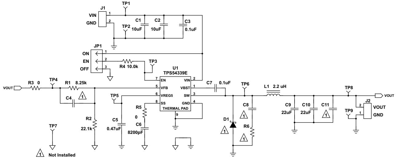
Figure 6-1. TPS54339EEVM-056 Schematic Diagram
