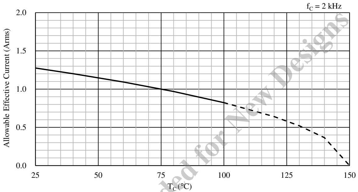
Figure 14-37. Allowable Effective Current ( f_c = 2\text{ kHz} ): SX68001MH
