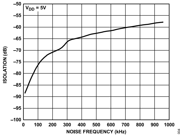
Figure 5. Channel-to-Channel Isolation
