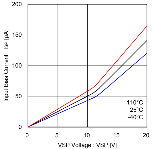
Figure 30. VSP Input Bias Current
