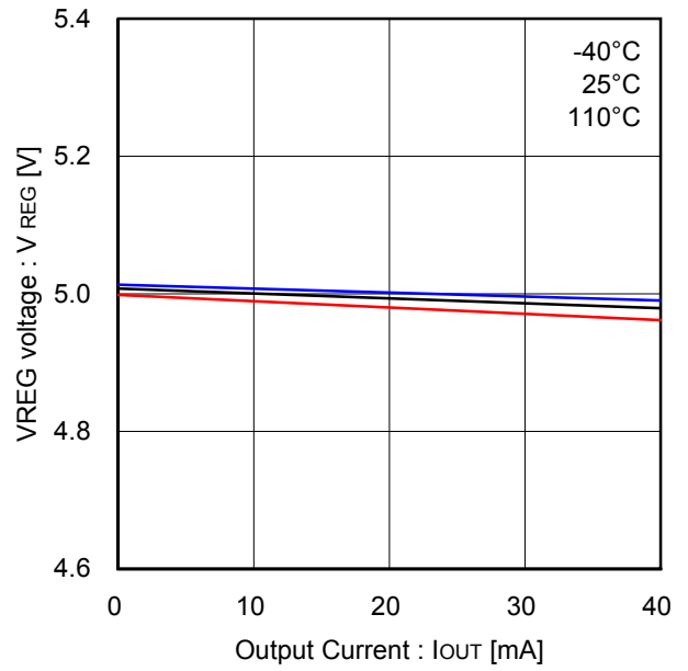
Figure 28. VREG Drive Capability
