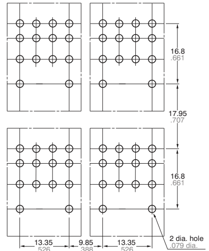
Side-by-side installation
