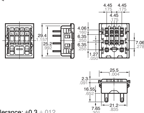
HC4-Socket (HC4-SS-K)
