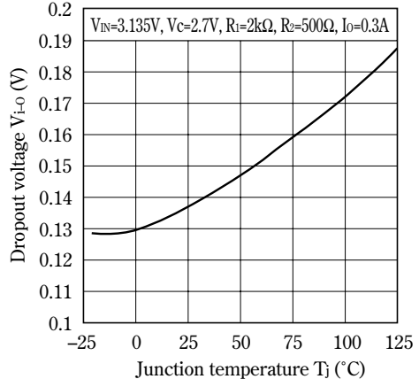
Fig.10 Dropout Voltage vs. Junction Temperature (PQ20WZ51)
