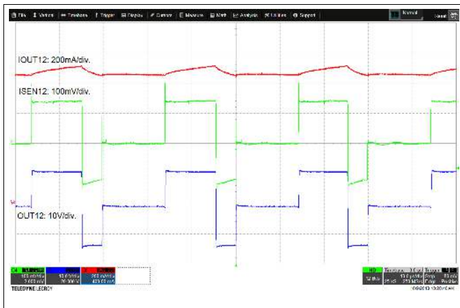
Figure 52. Zoomed Waveform Showing Current Regulation
