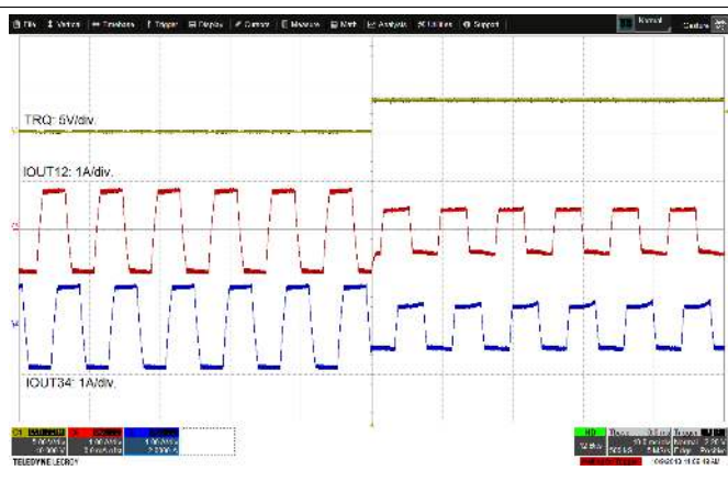
Figure 53. Torque Pin Functionality for Current Scaling
