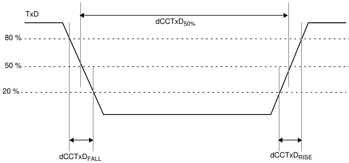
Figure 48. TxD signal
