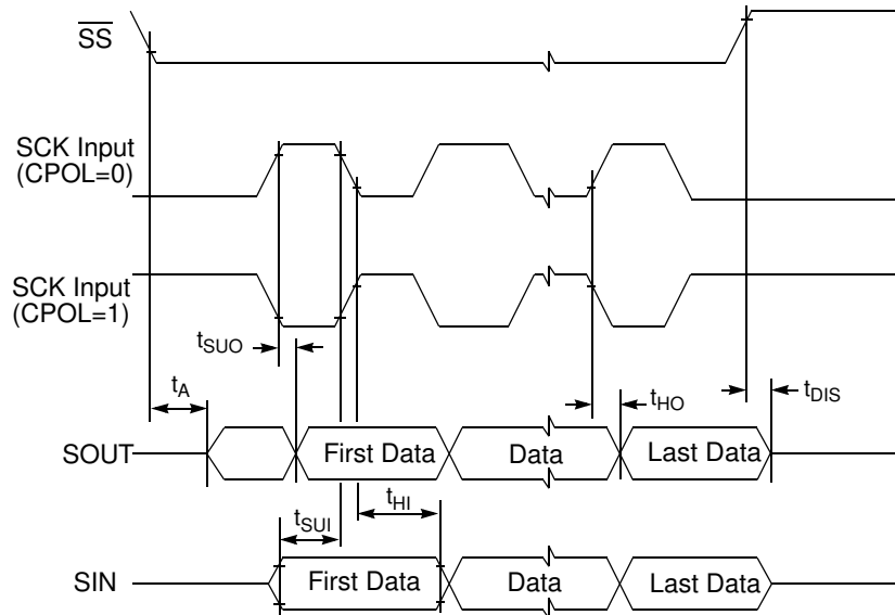
Figure 39. DSPI Slave Mode - Modified transfer format timing (MFTE = 0/1) — CPHA = 1
