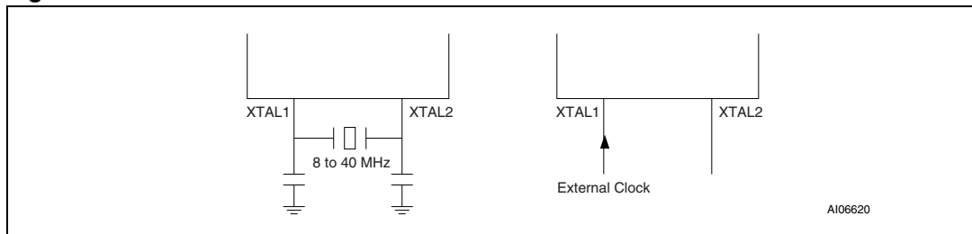
Figure 18. Oscillator
