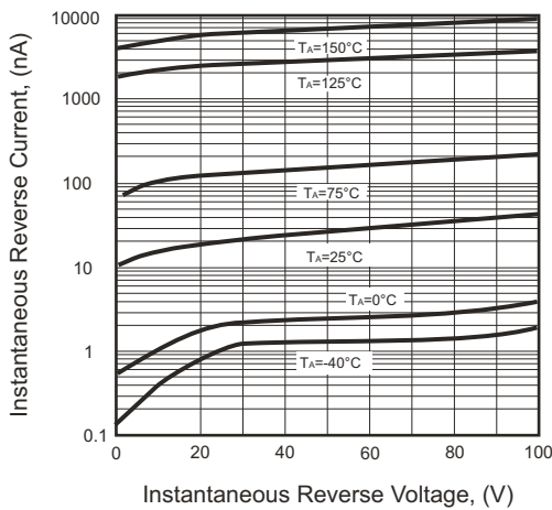
Fig.3 - Reverse Characteristics
