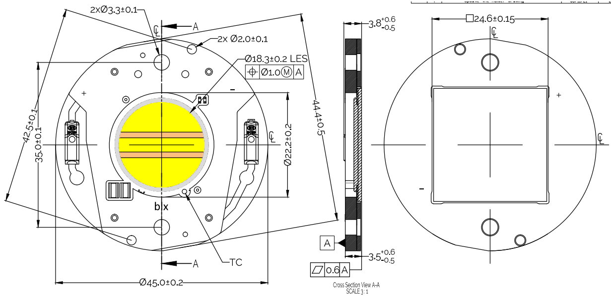
Figure 12: Mechanical Drawing Specification
