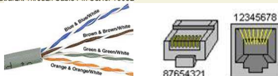
Straight-Through Cable Pin Out for T568B
