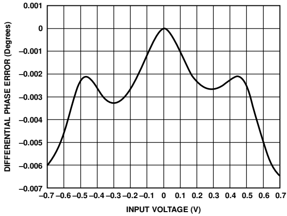
Figure 49. ADV3228 Differential Phase Error
