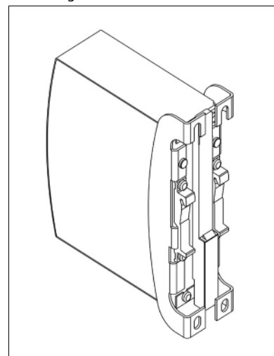
Fig. 23-3 Isometric view
