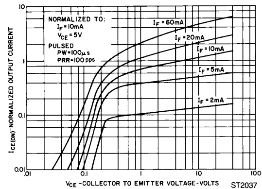
Fig. 4. Output Characteristics
