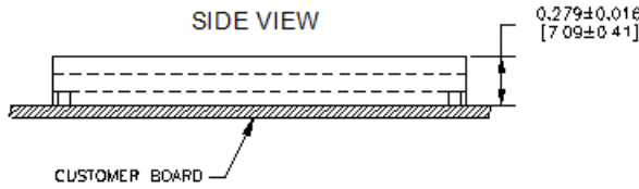
QMS48 (SurfaceMount)
