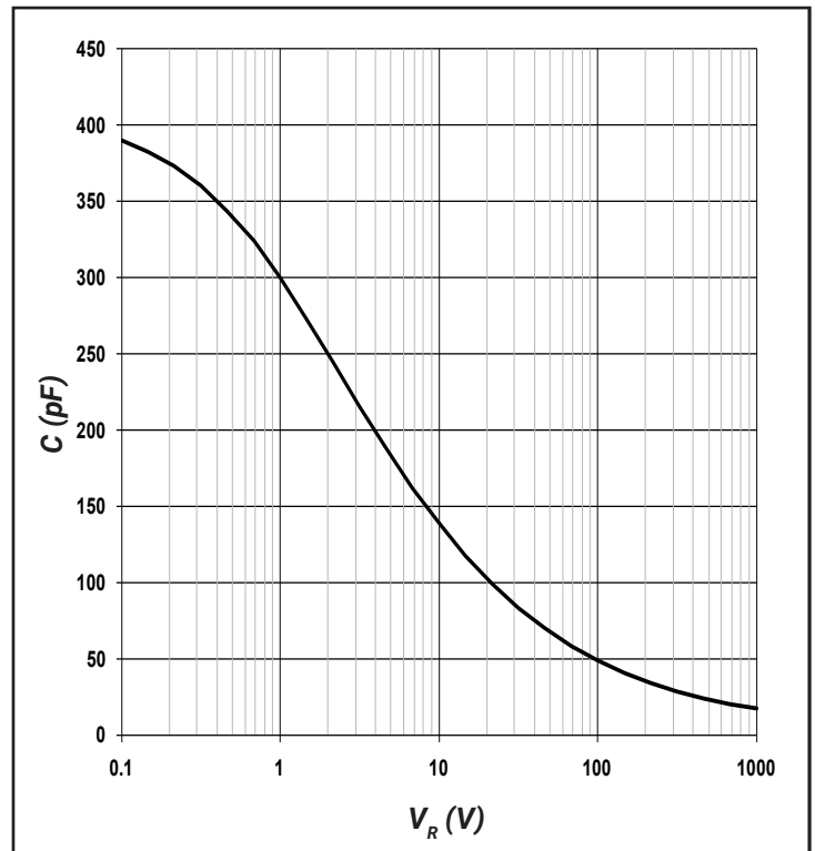
Figure 4. Capacitance vs. Reverse Voltage
