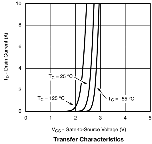
Transfer Characteristics
