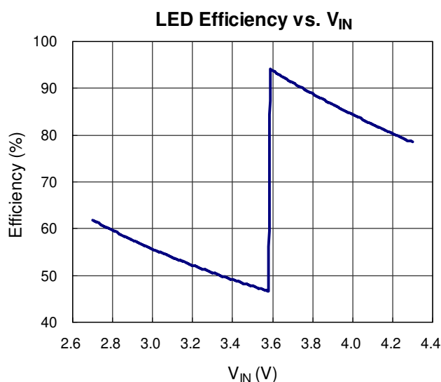
Figure 3. Efficiency of RT9363. ( I_{LED} = 60mA , V_F = 3.45V )
