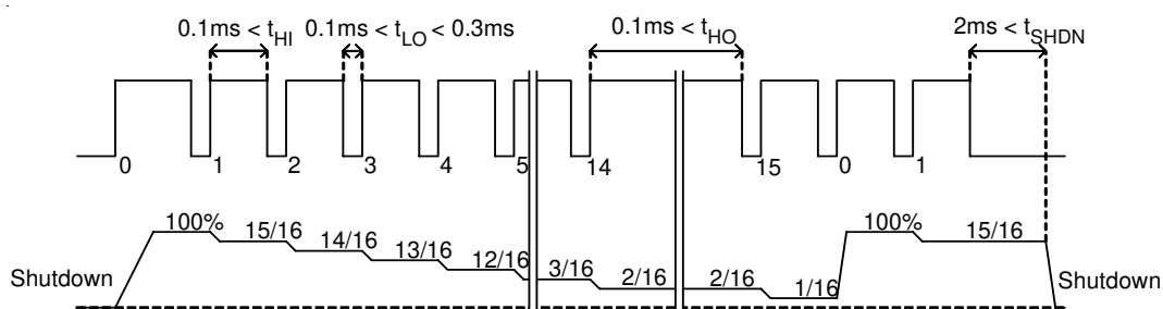
Figure 1. Brightness control by pulse dimming. RT9363 implements 16 steps brightness control
