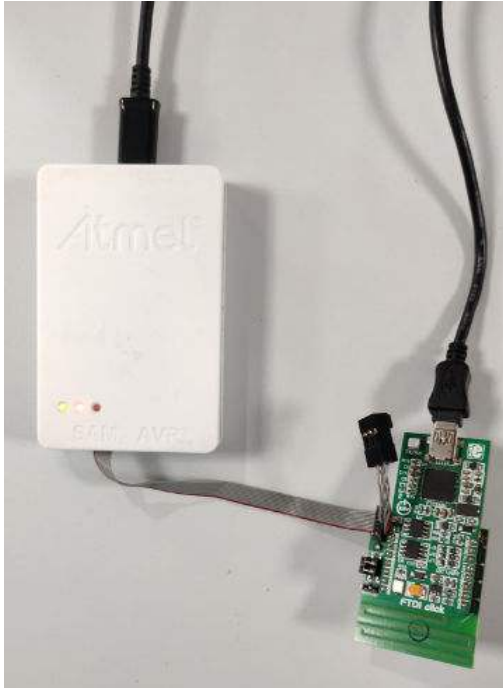
Figure 4-11. Connecting Programmer/Debugger with ATSAMR30M Sensor Board
