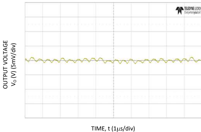
Figure 21. Typical output ripple ( C_o=4 \times 0.047 \mu\text{F} + 4 \times 0.1 \mu\text{F} + 15 \times 22 \mu\text{F} + 73 \times 47 \mu\text{F} + 6 \times 470 \mu\text{F} polymer, V_{IN} = 12\text{V} , I_o = I_{o,max} ).
