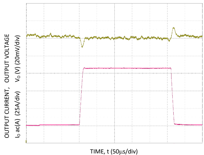
Figure 4. Trans. Resp. to 10A/μs Load Change from 25% to 75% at 12VIN, C_o=4 \times 0.047 \mu\text{F} + 4 \times 0.1 \mu\text{F} + 15 \times 22 \mu\text{F} + 73 \times 47 \mu\text{F} + 6 \times 470 \mu\text{F} polymer.
