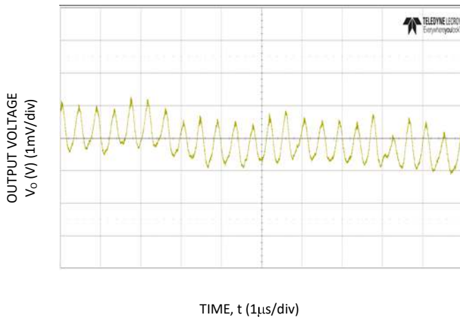
Figure 9. Typical output ripple ( C_o=4x0.047\mu F + 4x0.1\mu F + 15x22\mu F + 73x47\mu F + 6x470\mu F polymer, V_{IN} = 12V , I_o = I_{o,max} ).
