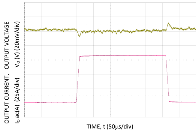
Figure 10. Trans. Resp. to 100A/μs Load Change from 25% to 75% at 12V IN , C_o=4x0.047\mu F + 4x0.1\mu F + 15x22\mu F + 73x47\mu F + 6x470\mu F polymer.
