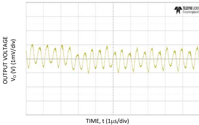
Figure 15. Typical output ripple ( C_o=4 \times 0.047 \mu\text{F} + 4 \times 0.1 \mu\text{F} + 15 \times 22 \mu\text{F} + 73 \times 47 \mu\text{F} + 6 \times 470 \mu\text{F} polymer, V_{IN} = 12\text{V} , I_o = I_{o,max} ).
