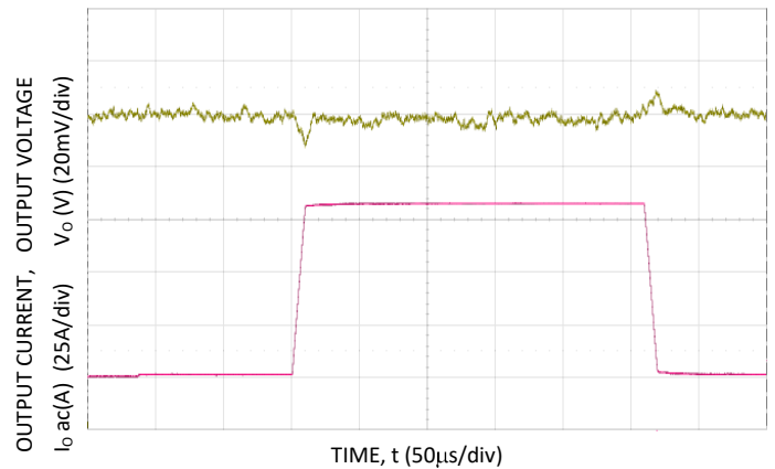
Figure 22. Trans. Resp. to 100A/μs Load Change from 25% to 75% at 12V IN , C_o=4 \times 0.047 \mu\text{F} + 4 \times 0.1 \mu\text{F} + 15 \times 22 \mu\text{F} + 73 \times 47 \mu\text{F} + 6 \times 470 \mu\text{F} polymer.
