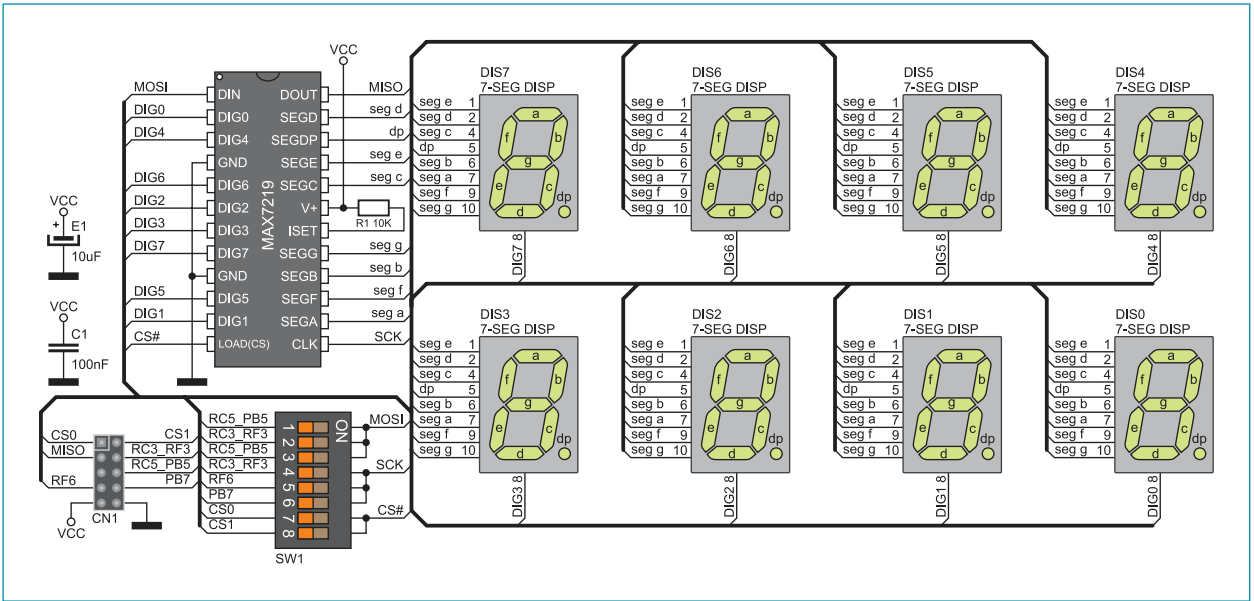
Figure 2: Serial 7-Seg Display 2 additional board connection schematic
