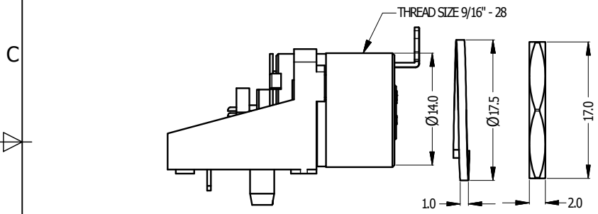
METAL WASHER
