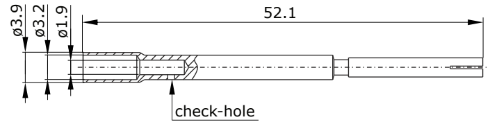
Main Dimensions contact socket
