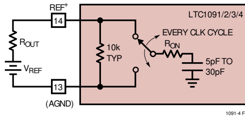
Figure 12. Reference Input Equivalent Circuit
