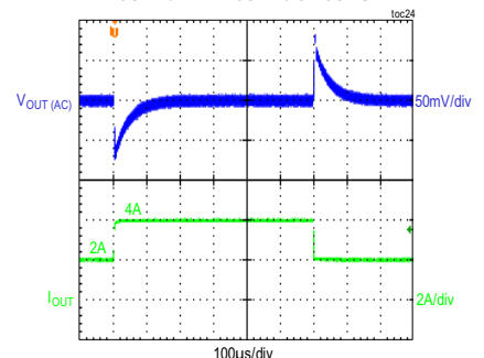
CONDITIONS: 3.3V OUTPUT, PWM/PM/DCM MODE
