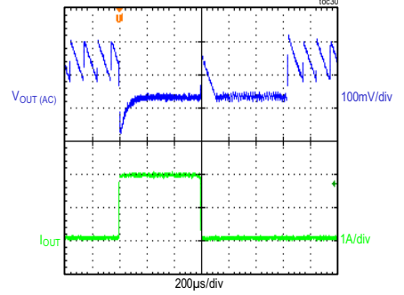
CONDITIONS: 5V OUTPUT, PFM MODE
