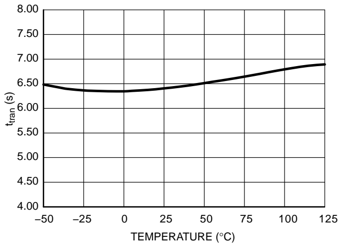
Figure 43. Transient Peak Power Timer Duration t_{tran} (NCP1240A/B only)
