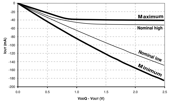
Figure 8: Pull-Up Characteristics
