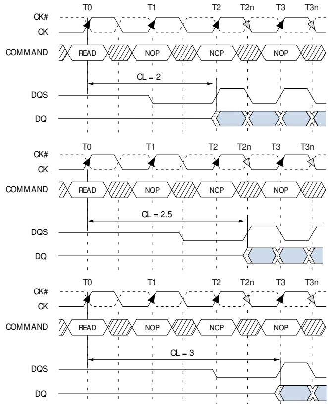
Figure 5: CAS Latency Diagram
