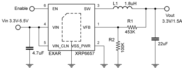
Fig. 22: Typical Application Circuit
