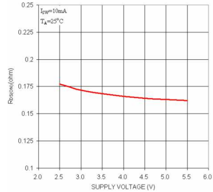
Fig. 13: NMOS R_{DS(ON)} vs Supply Voltage
