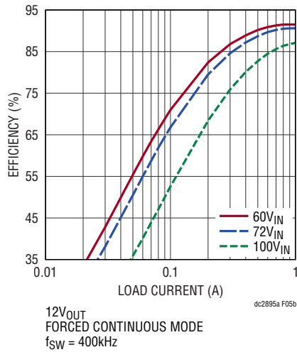
Figure 5. Efficiency at Various Input Voltages (Conditions: Forced Continuous Mode)
