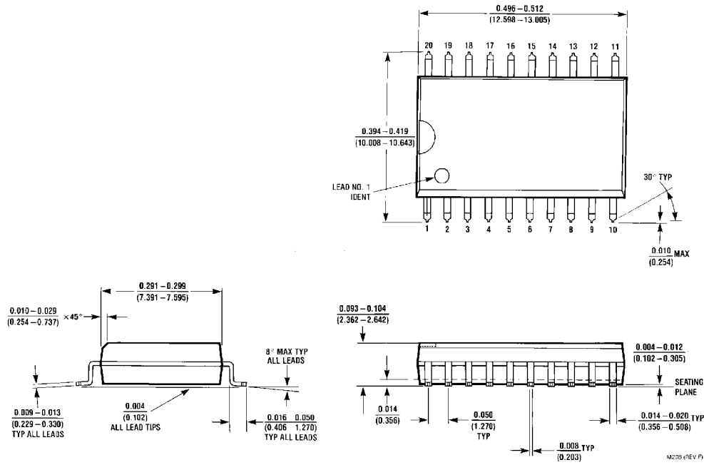
20-Lead Wide Small Outline Molded Package (M) Order Number DM74LS574WM Package Number M20B
