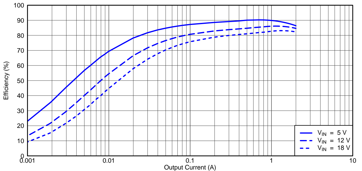
Figure 4. TPS54495EVM Converter 2 Light Load Efficiency
