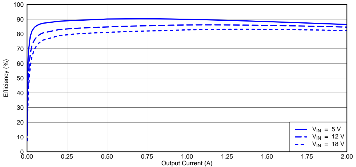
Figure 3. TPS54495EVM Converter 2 Efficiency
