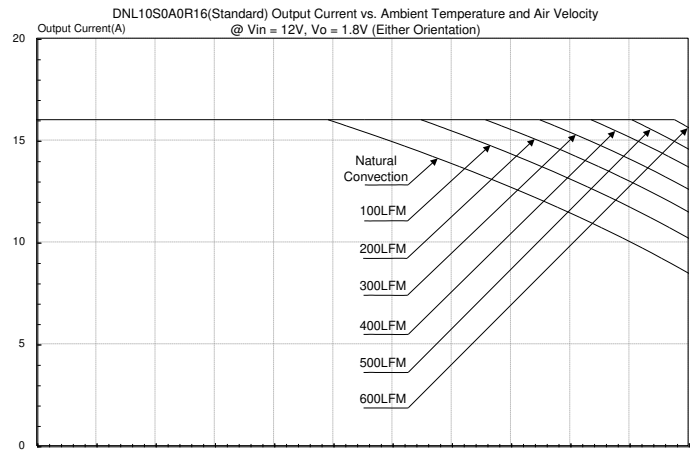
Figure 34: DNL10S0A0R16(Standard) Output current vs. ambient temperature and air velocity @ Vin=12V, Vout=1.8V(Either Orientation)
