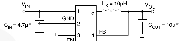
Figure 2. 5-Lead SOT-23
