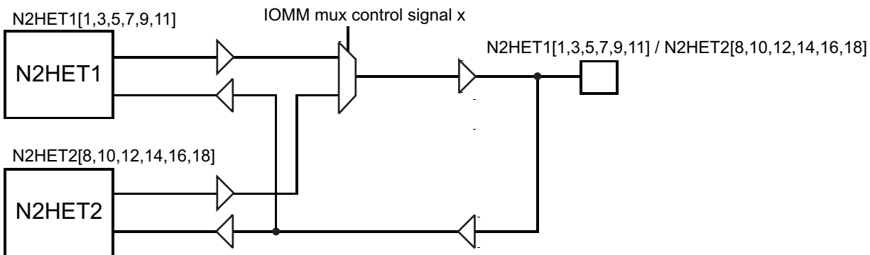
Figure 7-7. N2HET Monitoring
