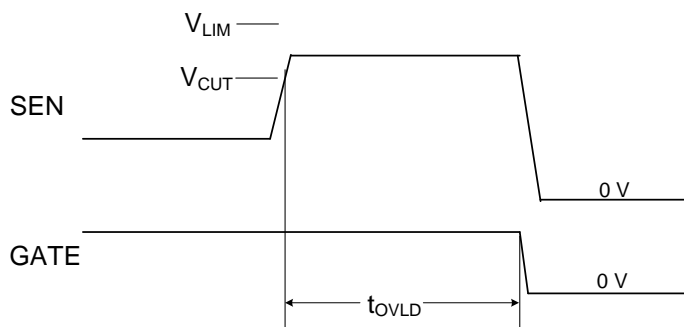
Figure 15. Overcurrent Fault Timing
