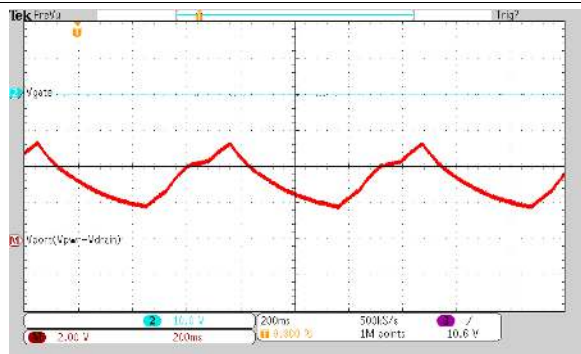
Figure 74. Detection With Invalid PD (15 kΩ and 0.1 μF)
