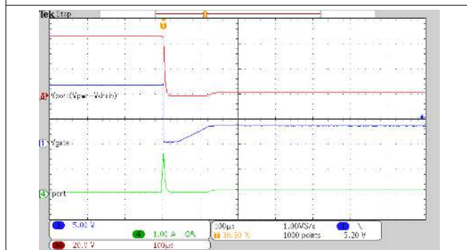
Figure 84. Rapid Response to a 1-Ω Short - PoE+ Mode
