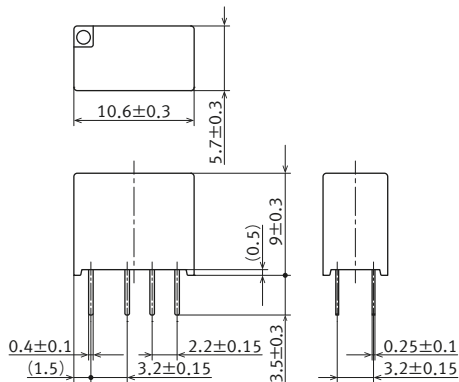
External dimensions
