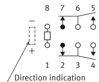
Schematic ( TOP VIEW ) Single side stable High sensitivity single side stable ( De-energize )
