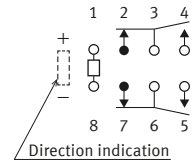
Schematic ( BOTTOM VIEW ) Single side stable High sensitivity single side stable ( De-energize )
