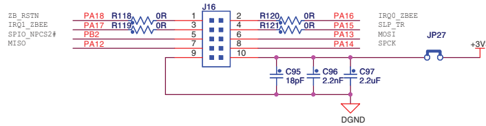
Figure 4-23. ZigBEE Interface
